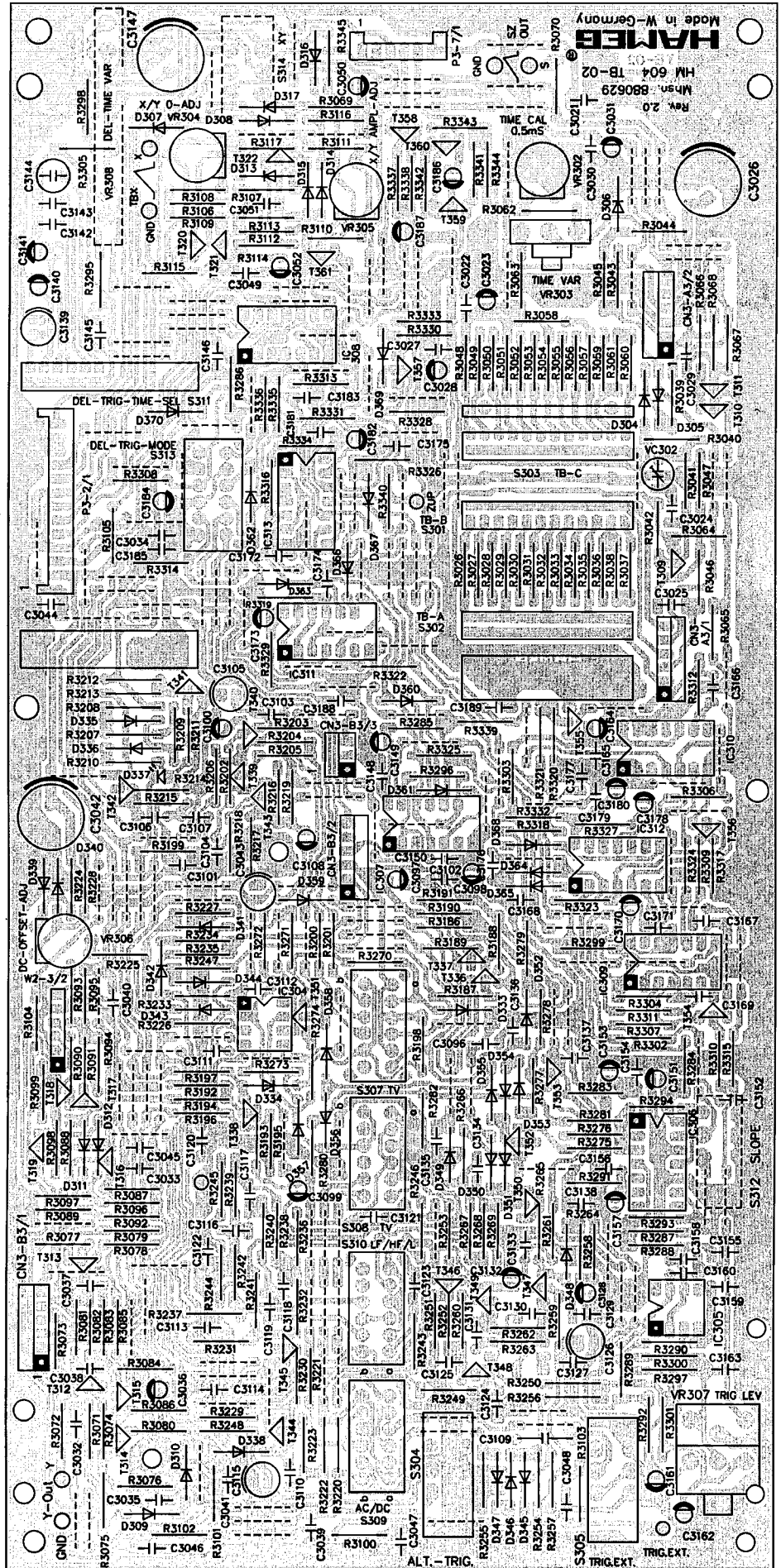
TB-2 Board
